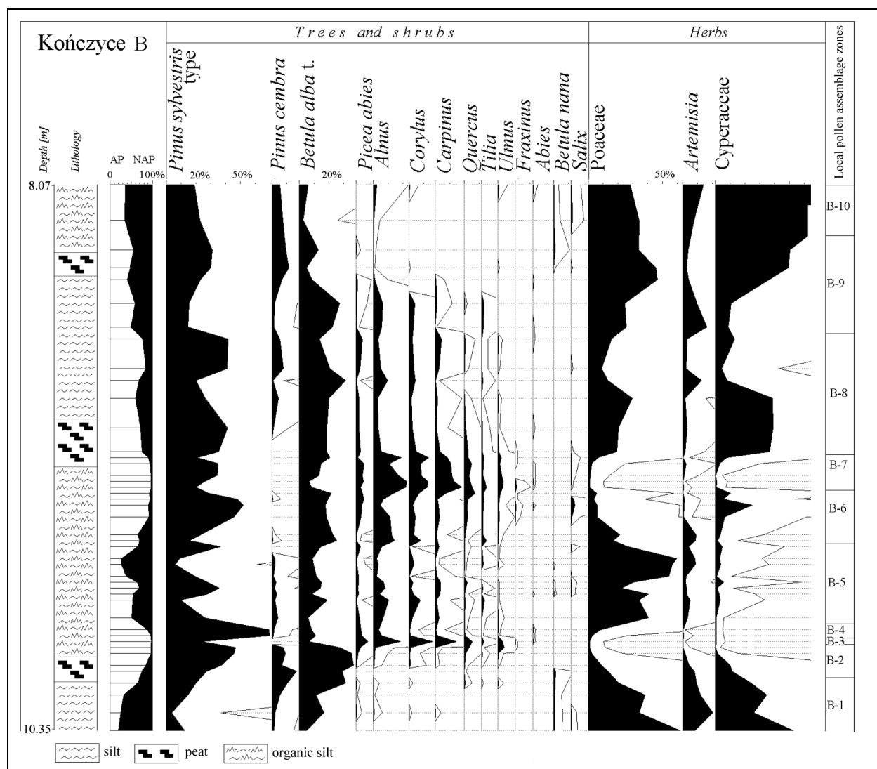
Fig. 6. The simplified pollen diagram of the Kończyce Wielkie site 4–B profile.
